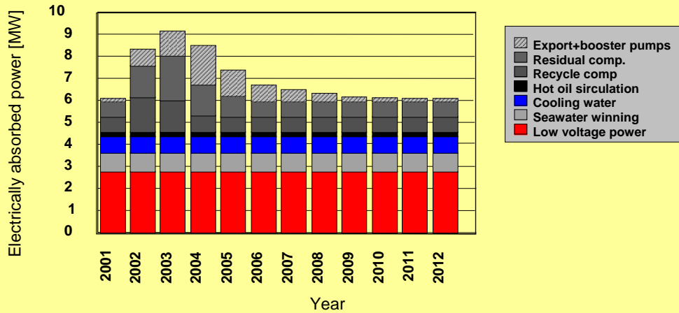
Prognosis of electrical power consumed on Heimdal Platform
